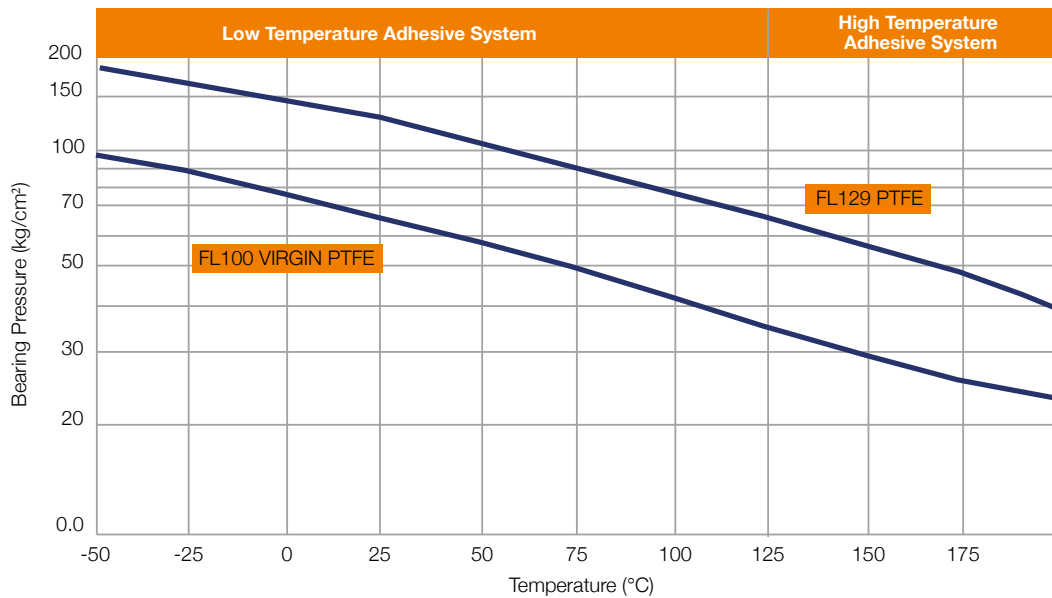
Recommended maximum Bearing Pressure against Temperature
