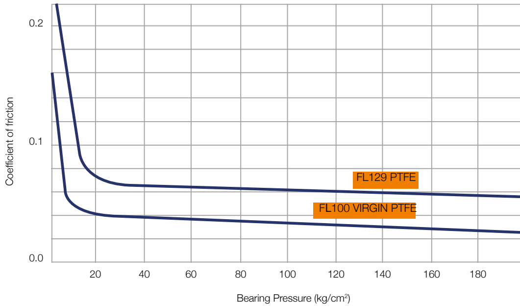
Coefficient of friction: Effect of Load
