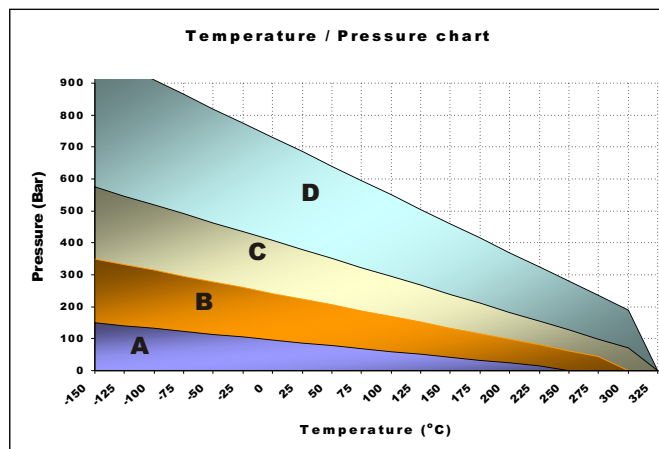
Figure 1, Temperature/Pressure Chart
